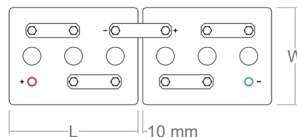
6V 4 OGi 100-N6 to 6V 12 OGi 300-N6
